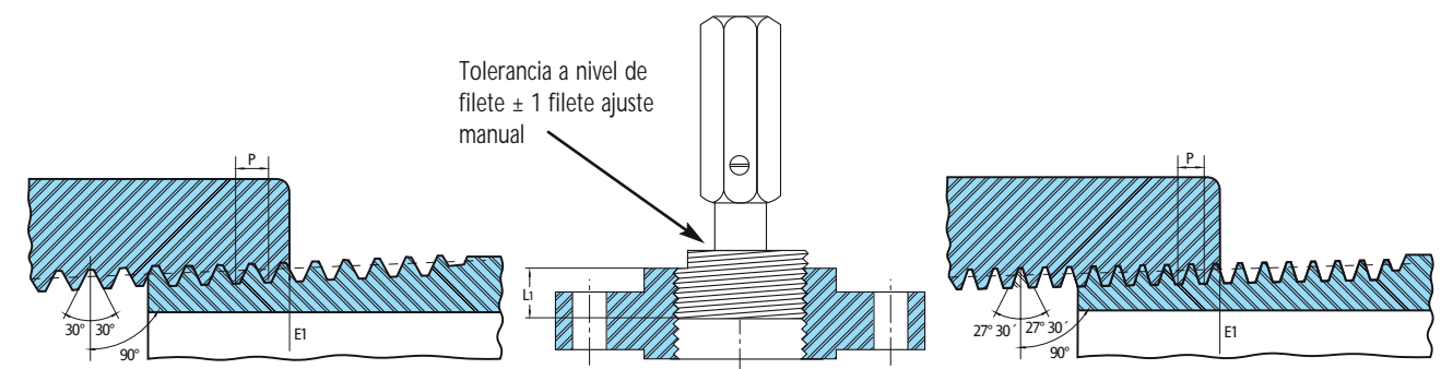
BRITISH STANDARD PIPE THREAD (BSPT)=DIN 2999=IRAM 5063= NM-ISO 7-1 AMERICAN STANDARD B1.20 (NPT) Tabla 09
